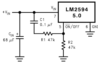
Figure 22. Delayed Startup
