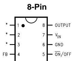
Figure 1. Top View
