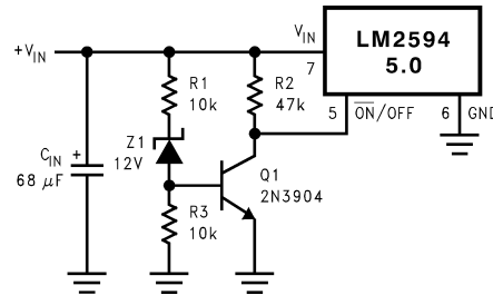
Figure 23. Undervoltage Lockout for Buck Regulator
