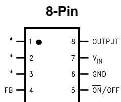
Figure 2. Top View
