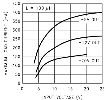
Figure 27. Inverting Regulator Typical Load Current
