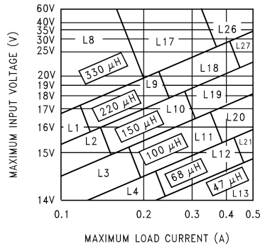
Figure 10. LM2594/LM2594HV-12
