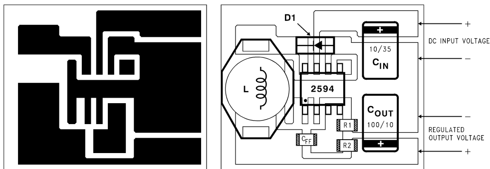
Figure 33. PC Board Layout
