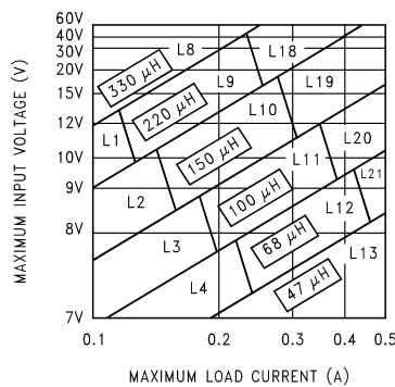
Figure 9. LM2594/LM2594HV-5.0
