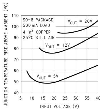
Figure 20. Junction Temperature Rise, SO-8
