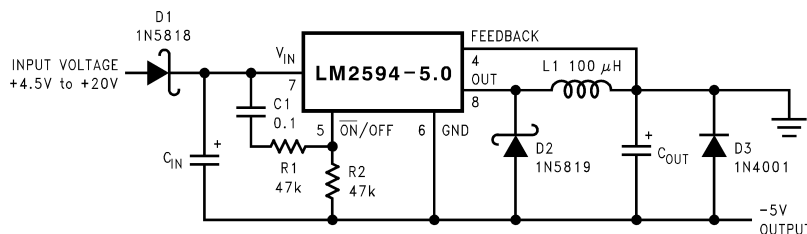
Figure 25. Undervoltage Lockout with Hysteresis for Inverting Regulator
