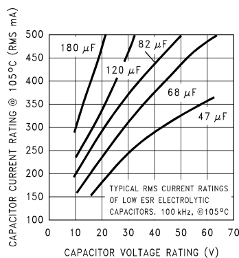
Figure 12. RMS Current Ratings for Low ESR Electrolytic Capacitors (Typical)
