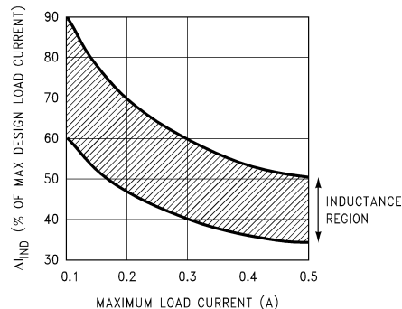
Figure 15. ( \Delta I_{IND} ) Peak-to-Peak Inductor Ripple Current (as a Percentage of the Load Current) vs Load Current
