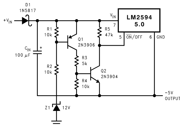
Figure 24. Undervoltage Lockout for Inverting Regulator
