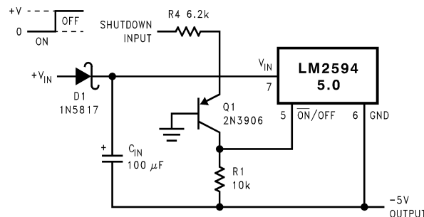
Figure 28. Inverting Regulator Ground Referenced Shutdown
