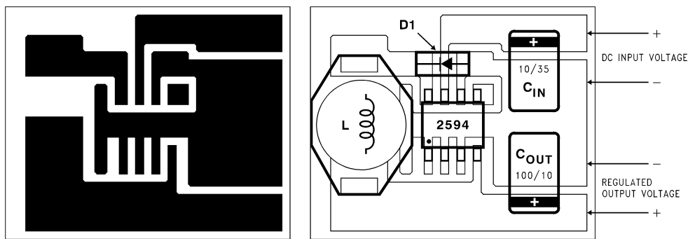
Figure 31. PC Board Layout
