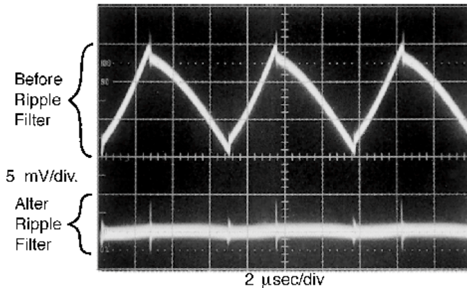
Figure 16. Post Ripple Filter Waveform
