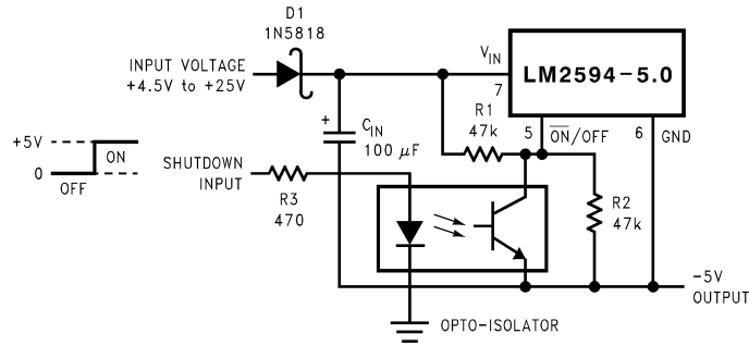
Figure 29. Inverting Regulator Ground Referenced Shutdown using Opto Device
