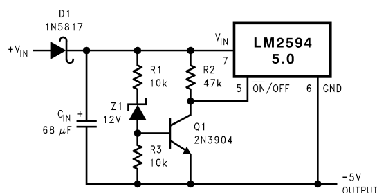
Figure 24. Undervoltage Lockout for Inverting Regulator
