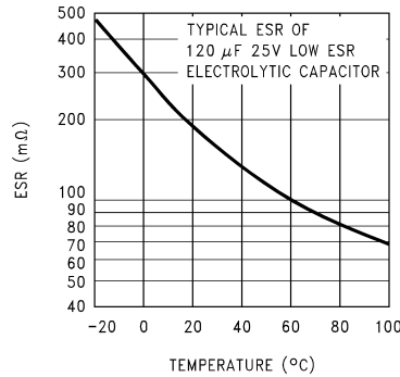
Figure 14. Capacitor ESR Change vs Temperature
