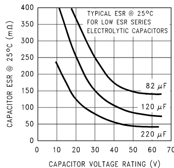
Figure 13. Capacitor ESR vs Capacitor Voltage Rating (Typical Low ESR Electrolytic Capacitor)
