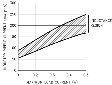
Figure 17. Peak-to-Peak Inductor Ripple Current vs Load Current
