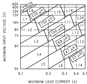
Figure 8. LM2594/LM2594HV-3.3
