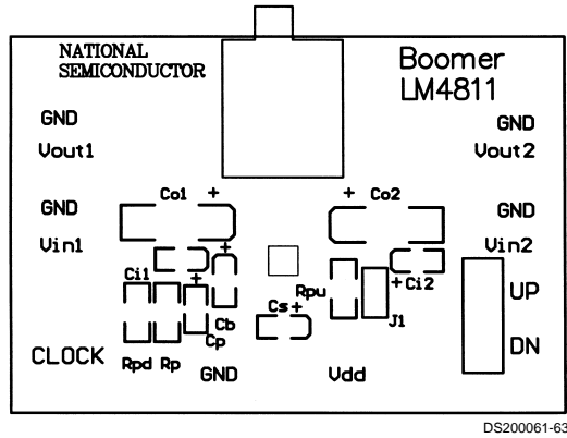
Figure 7. Recommended LD PC Board Layout: TOP Silk Screen
