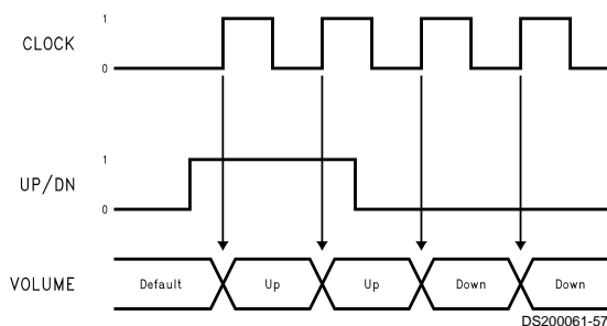
FIGURE 2. Timing Diagram
