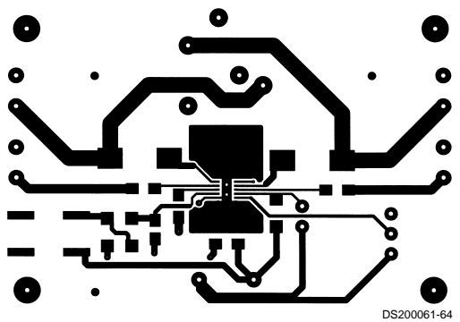
Figure 8. Recommended LD PC Board Layout: TOP Top Layer
