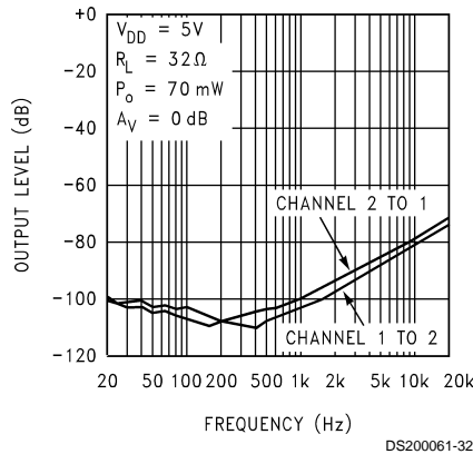
Channel Separation
