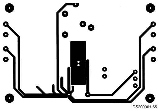
Figure 9. Recommended LD PC Board Layout: Bottom Layer
