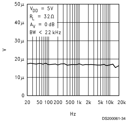
Noise Floor
