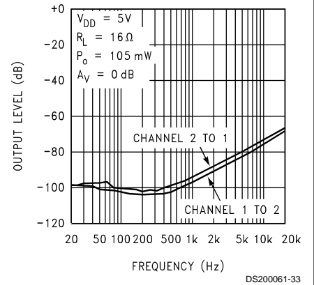
Channel Separation
