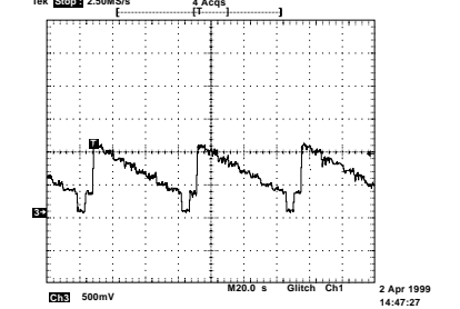
IC301 Pin 145, Luminance (Super video out Mode)
