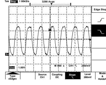
IC301 Pin 159, MPEG Clock(27MHz)
